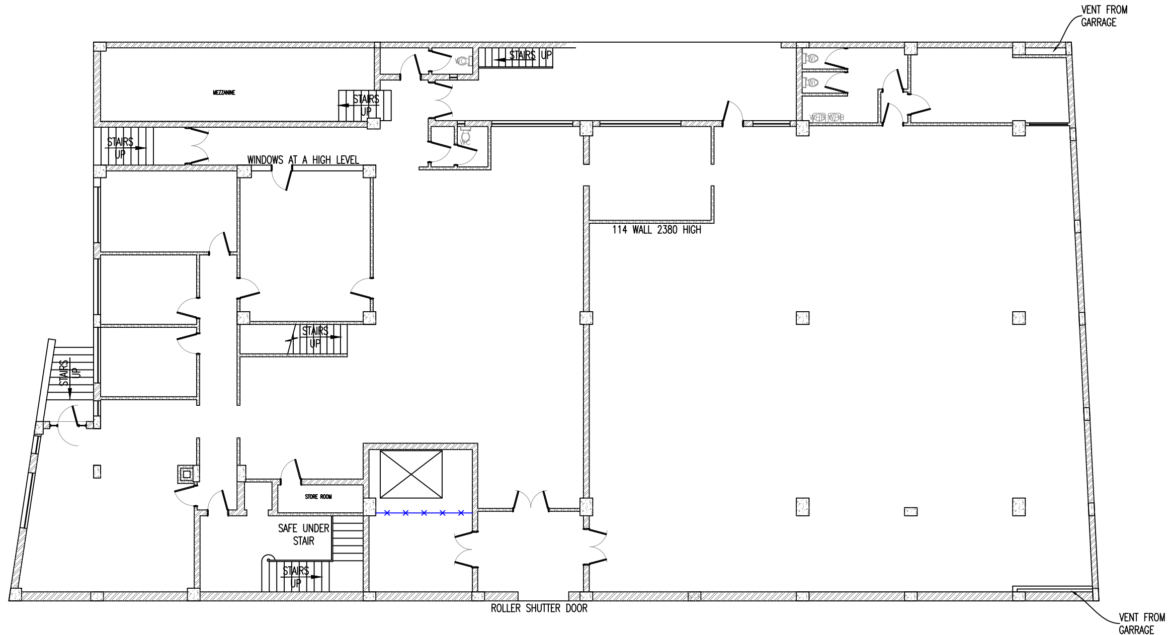
PLAN ON GROUND FLOOR
