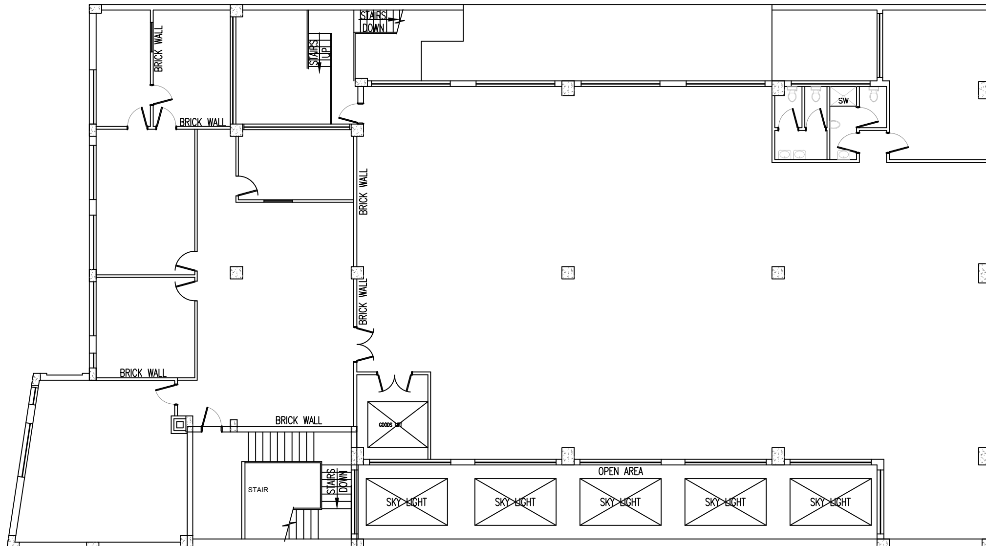
PLAN ON FIRST FLOOR
